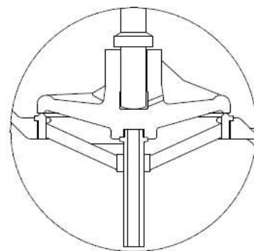
Screw-down check valve
